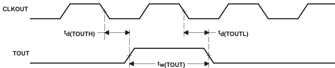
Figure 20. TOUT Timing
